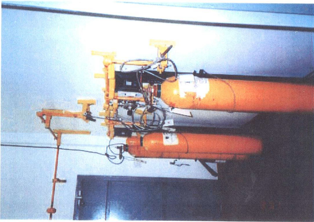
Photograph 3 : Draw-off Point in Chlorination Room 1
